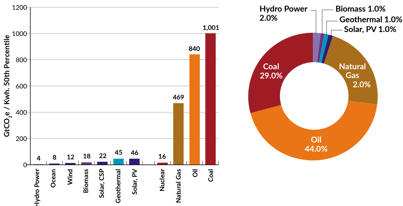
FIGURE 14: GHG Emissions of Alternative Energy Sources Per Unit of Energy and Shares of Different Energy Sources in Total Energy Supply in Indonesia (2015)
