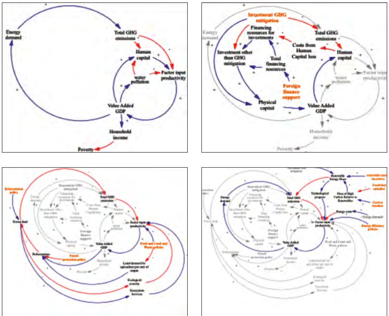
FIGURE 59: System Dynamics Representation of Indonesia Vision 2045
