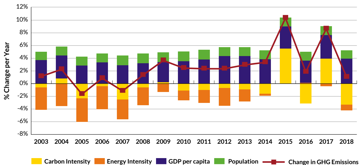
FIGURE 15A: Kaya Decomposition (from 3-year average data) (2000–2015)
