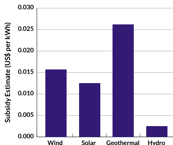
FIGURE 26: Subsidy Estimate of Recent Power Purchase Agreements (2016–17)
