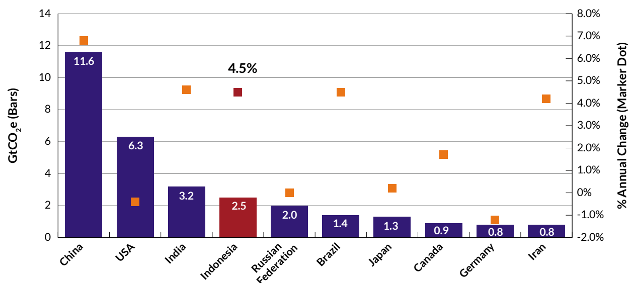
FIGURE 12A: Top 10 World Emitters of GHG (2014) and Annual Percent Change in GHG (2000–2014)
