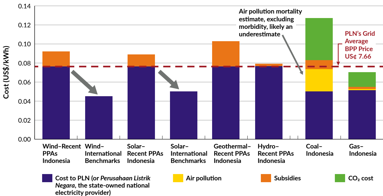
FIGURE 4: Relative Cost of Coal and Renewable Sources of Energy
