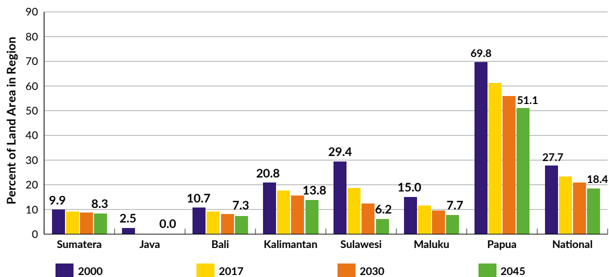
FIGURE 40: Land-use Change: Primary Forest Cover Proportion (Base Case)
