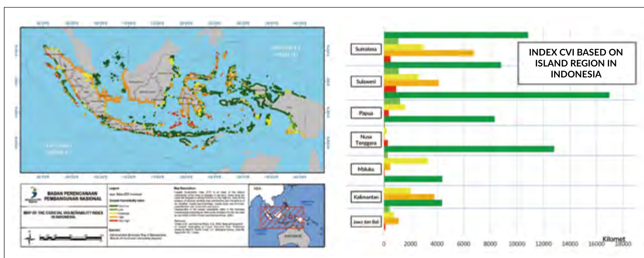
FIGURE 36: Map of Coastal Vulnerability and the Coastal Vulnerability Index (CVI) in Indonesia, Derived from RCP 4.5
