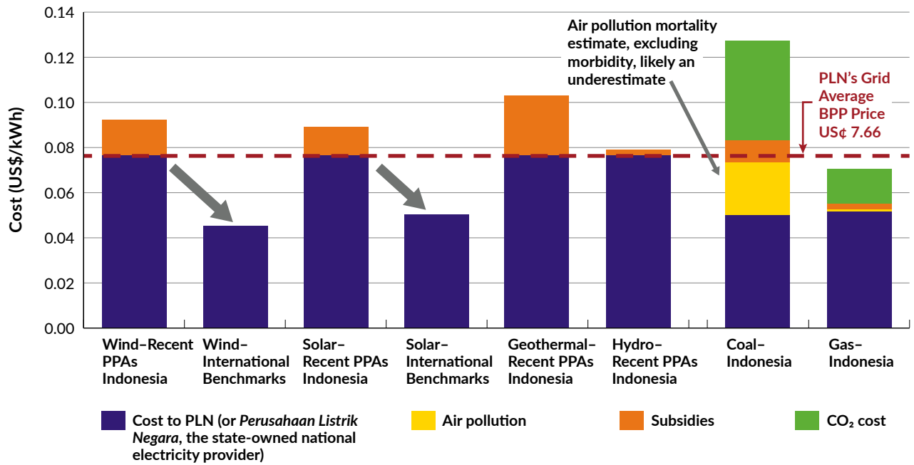
FIGURE 27: Cost Comparison for Electricity Production Sources in Indonesia, 2018
