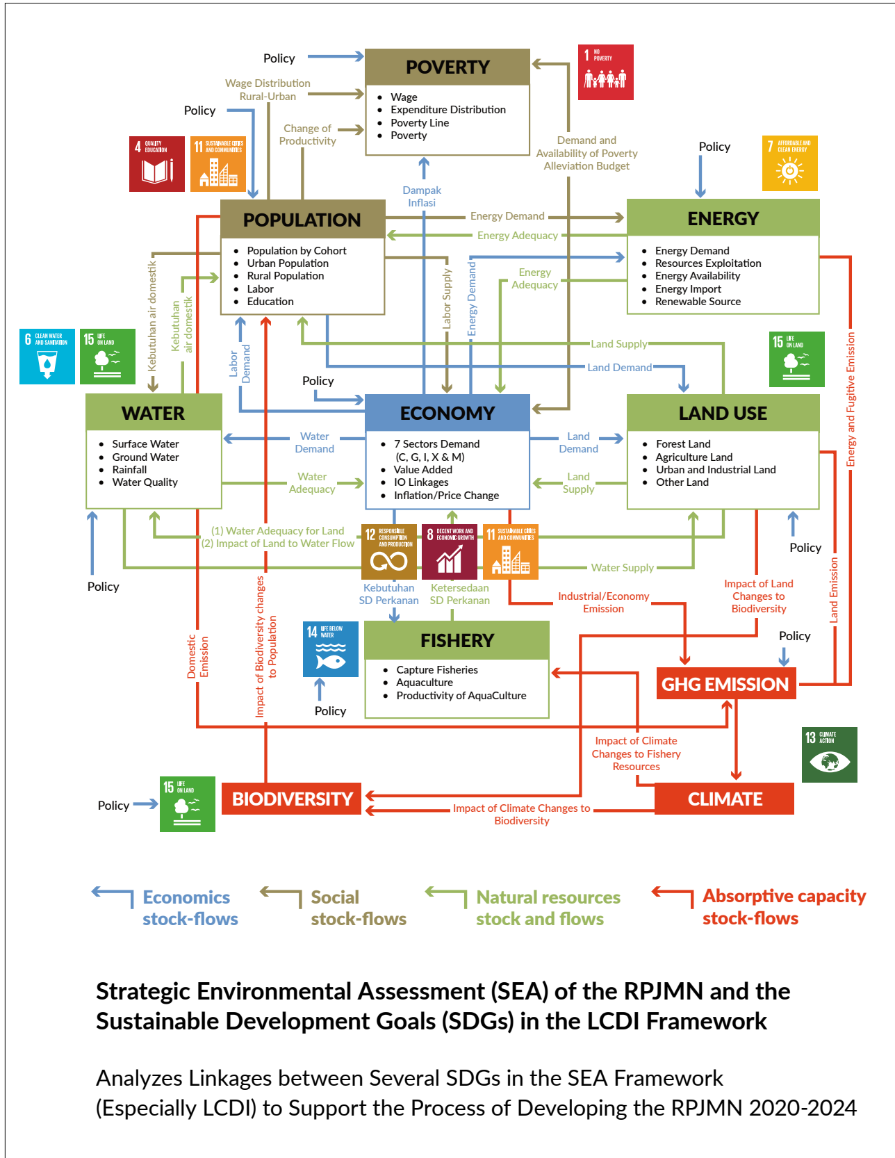
FIGURE 19: A High-Level Representation of IV2045
