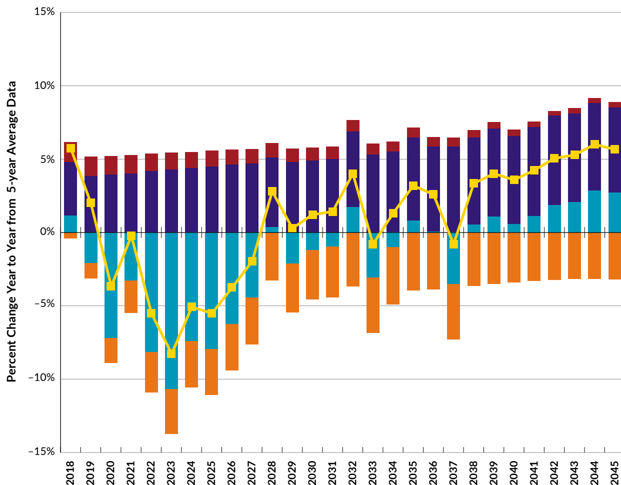
FIGURE 53: Kaya Decomposition: LCDI High (From 5-year Average Data) 2018–2045
