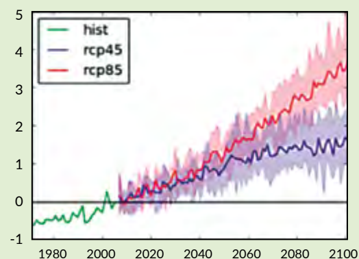
FIGURE 37: Projected Changes in Temperature for RCP 4.5 and RCP 8.5 relative to year 2000
